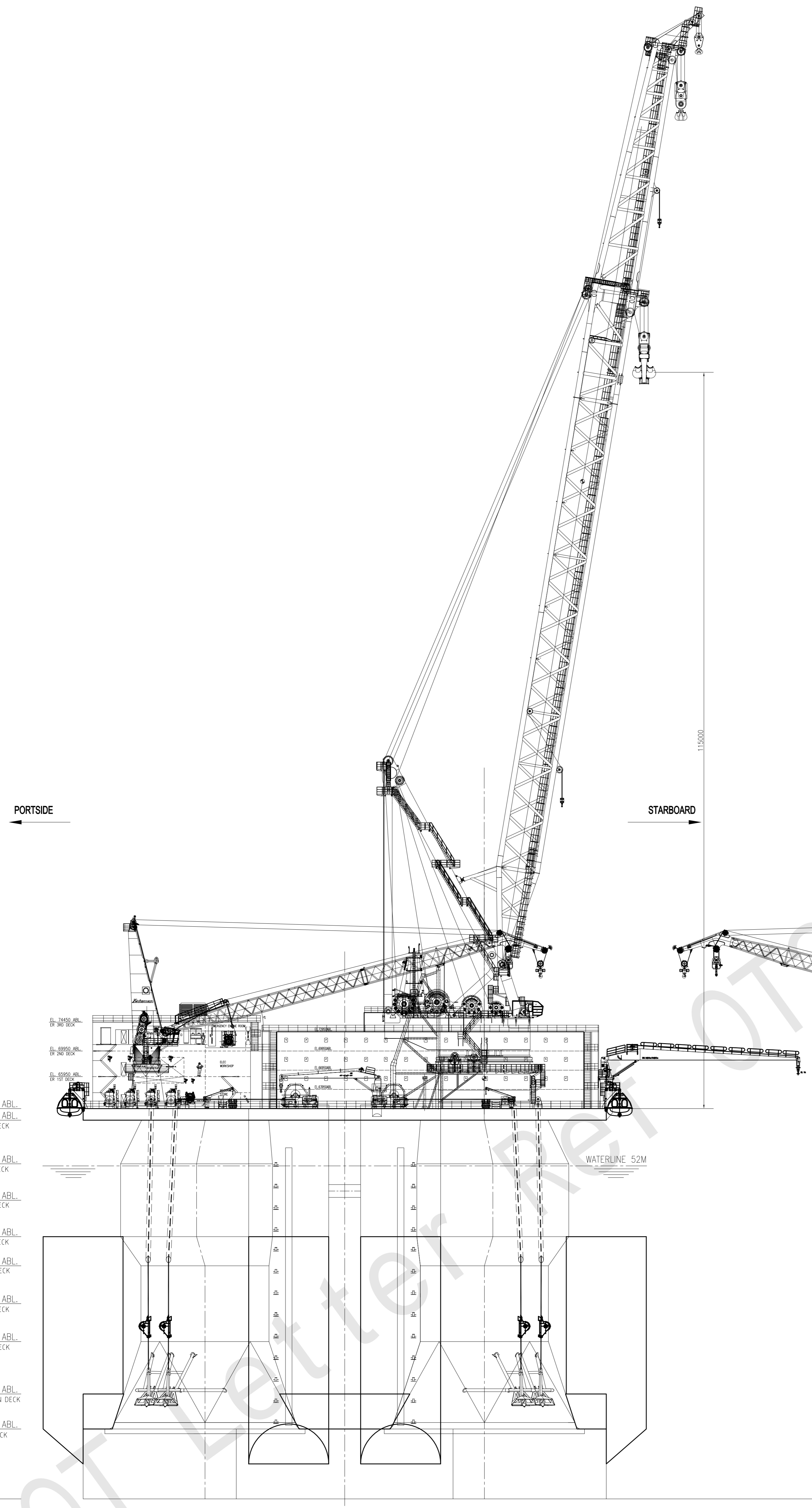
VIEW E LOOKING FACE TO COLUMN 1
