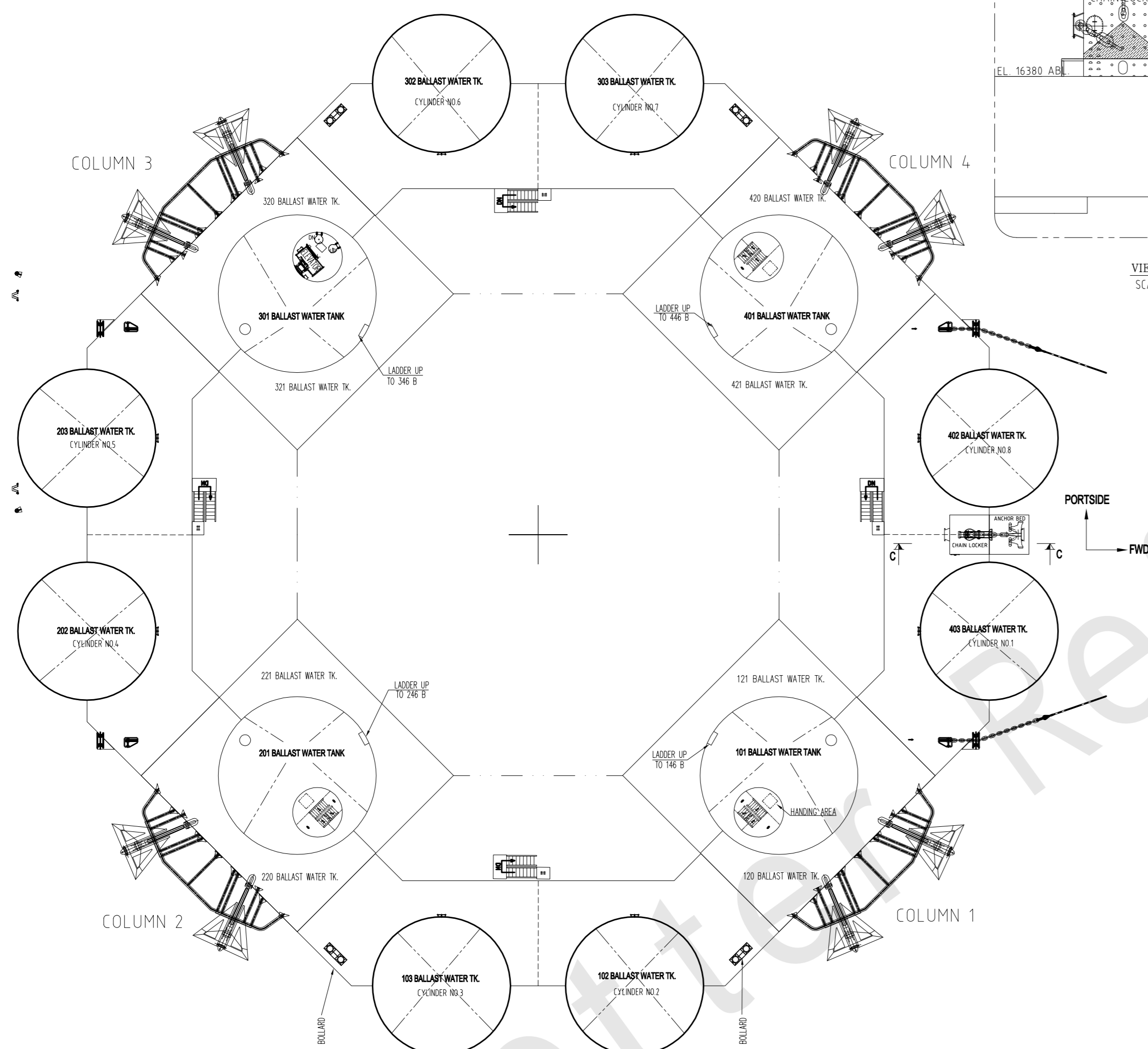
PLAN VIEW AT 16380
