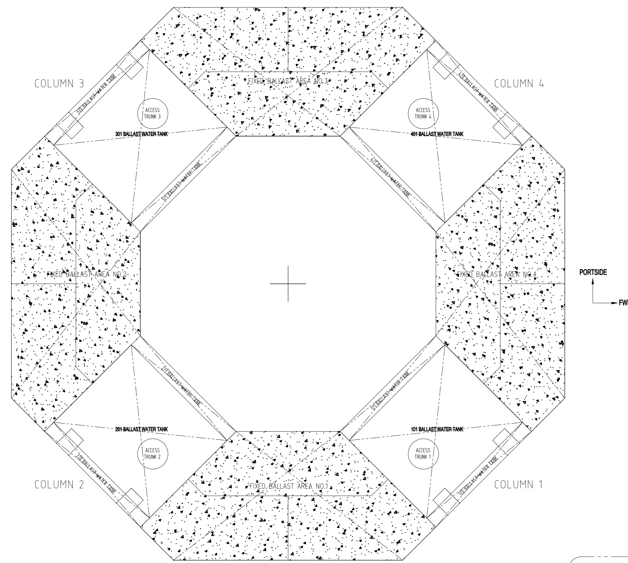
BOTTOM PLAN VIEW FIXED-BALLAST TOP AT EL. 500ABL
