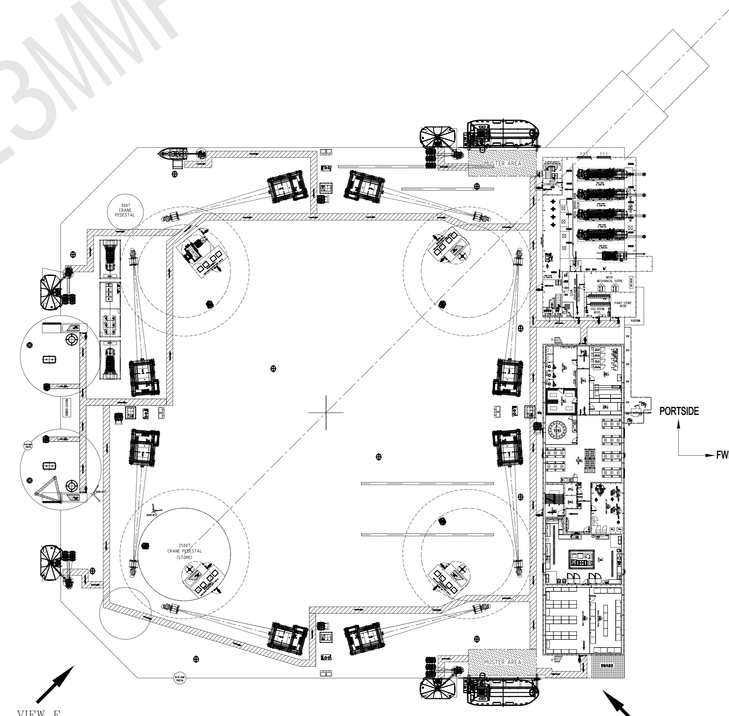
PLAN VIEW AT 60950 UPPER DECK
