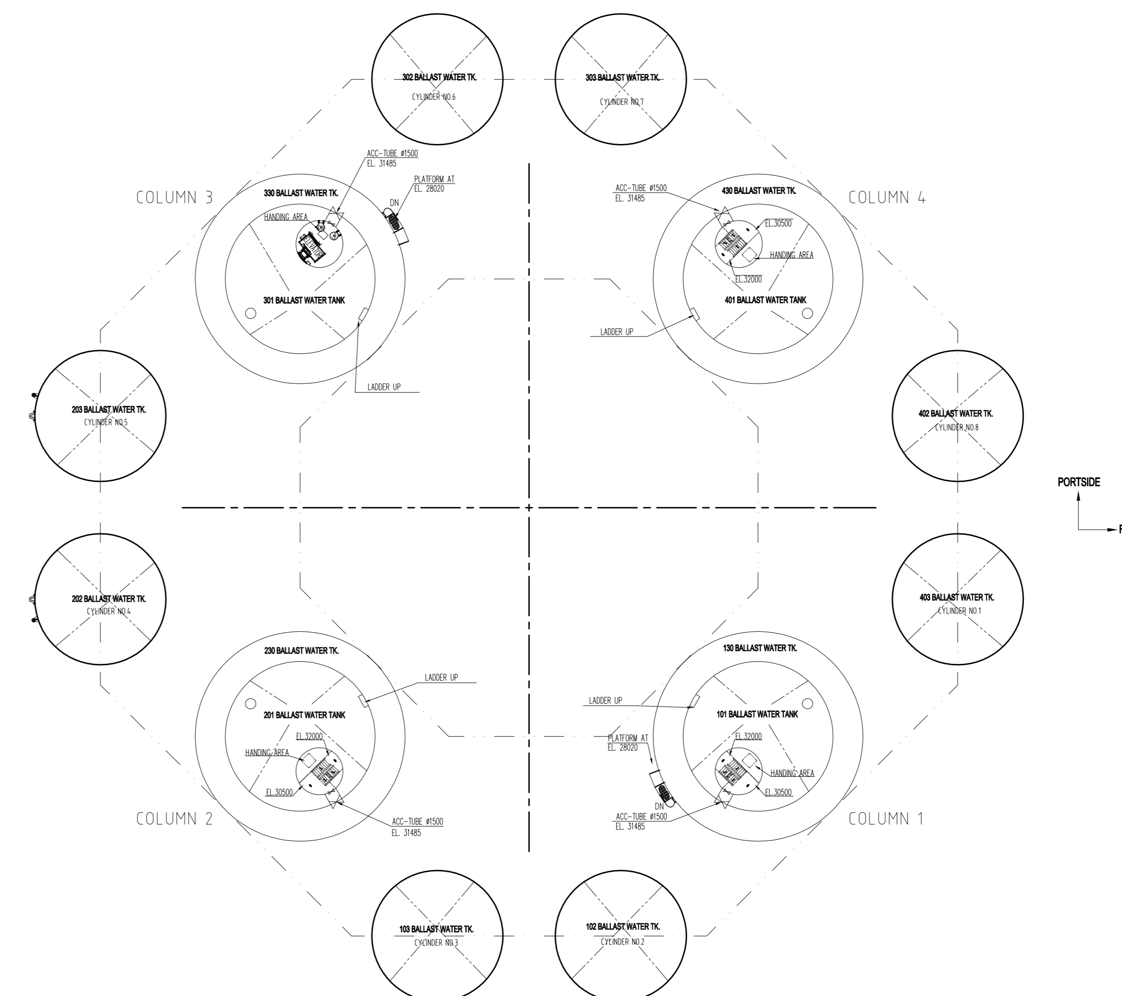
PLAN VIEW AT 30485 COLUMN 03 DECK
