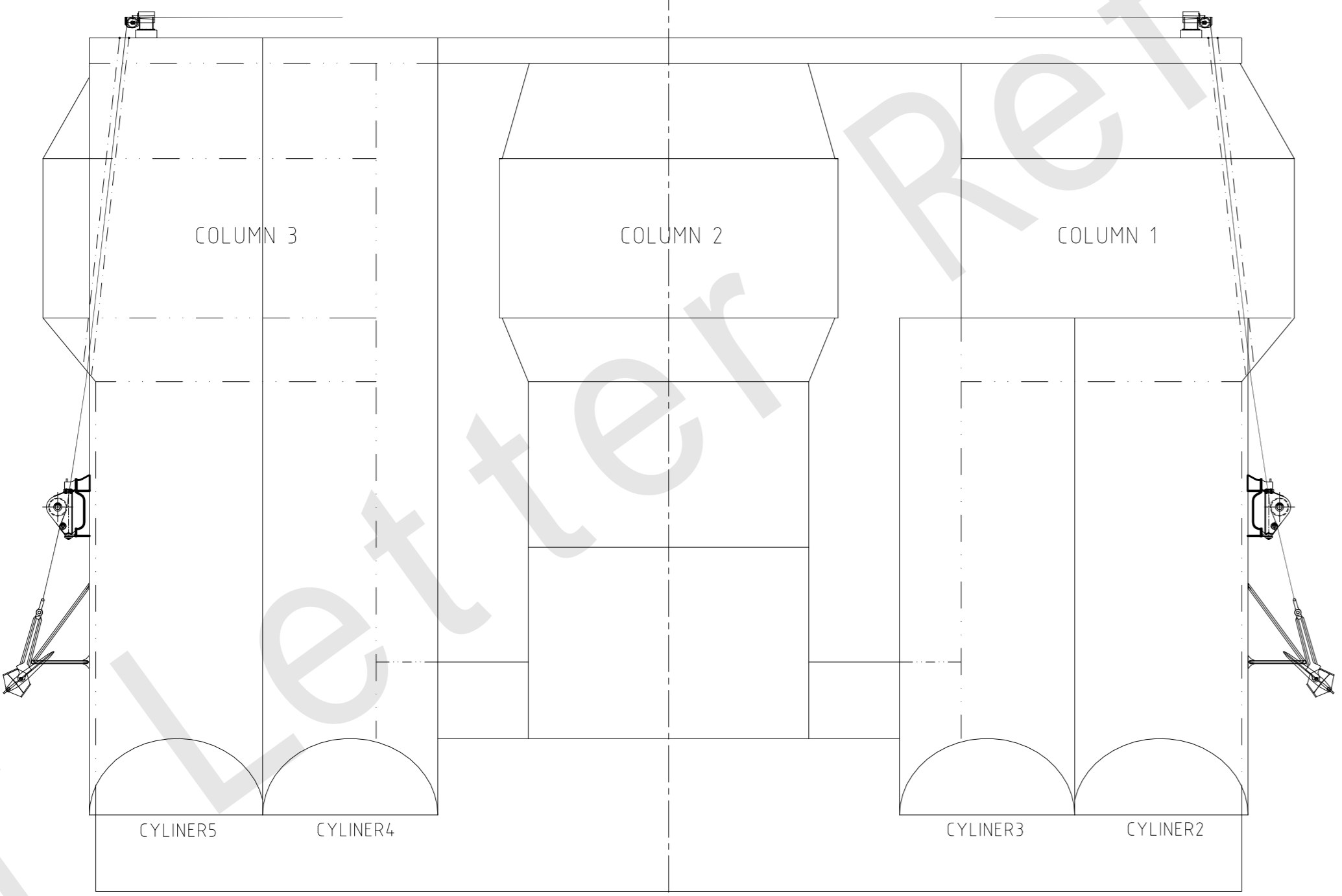
VIEW F LOOKING FACE TO COLUMN 2
