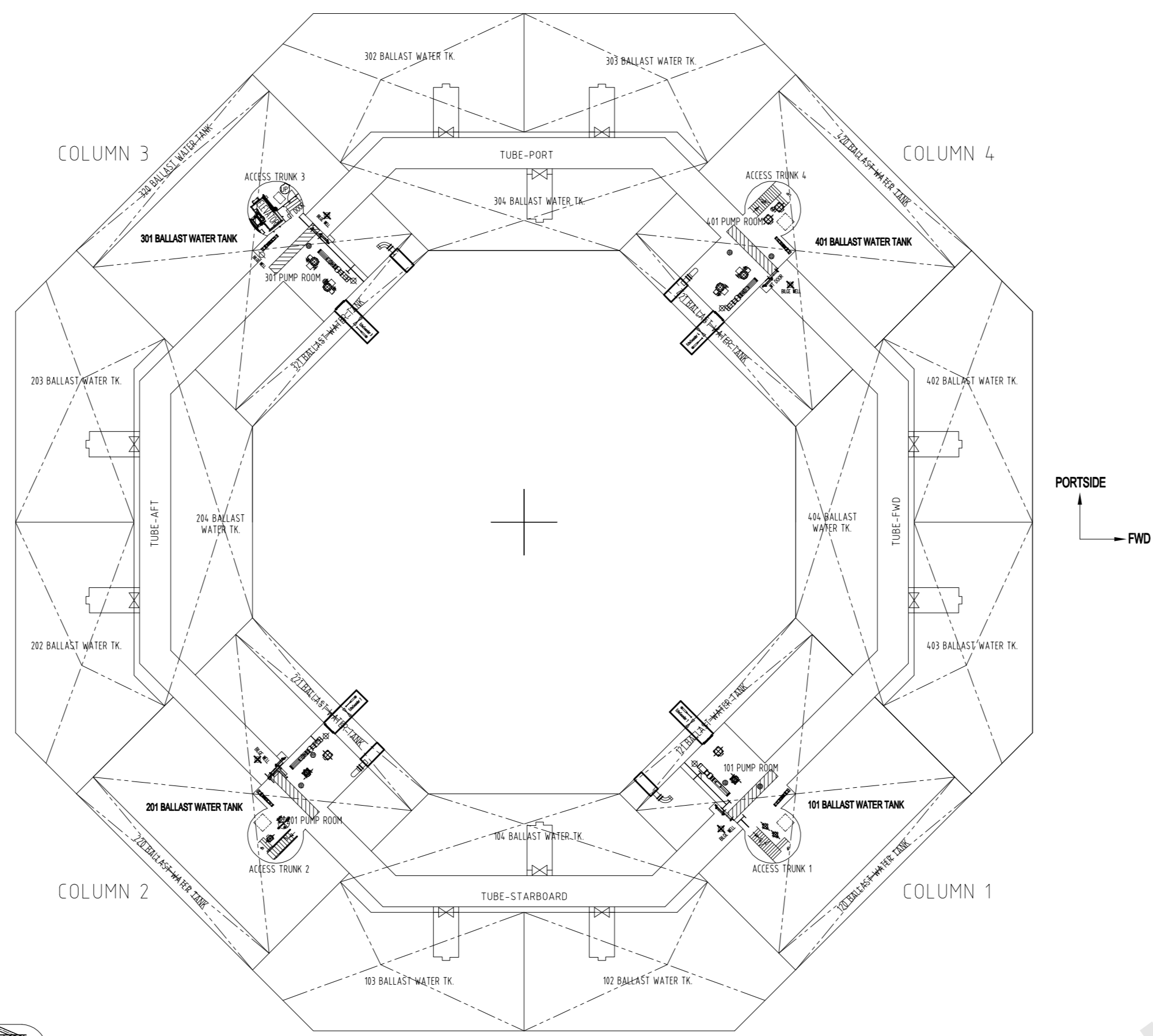
PLAN VIEW AT 3650
